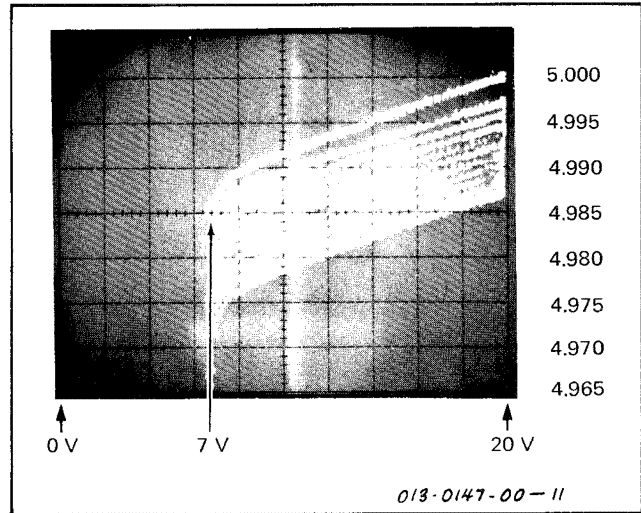
Fig. 2-15. Illustration of dropout voltage test, part h.
