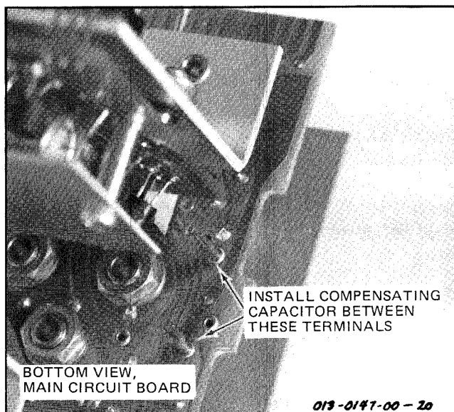
Fig. 2-5. Location of compensating capacitor terminals.
